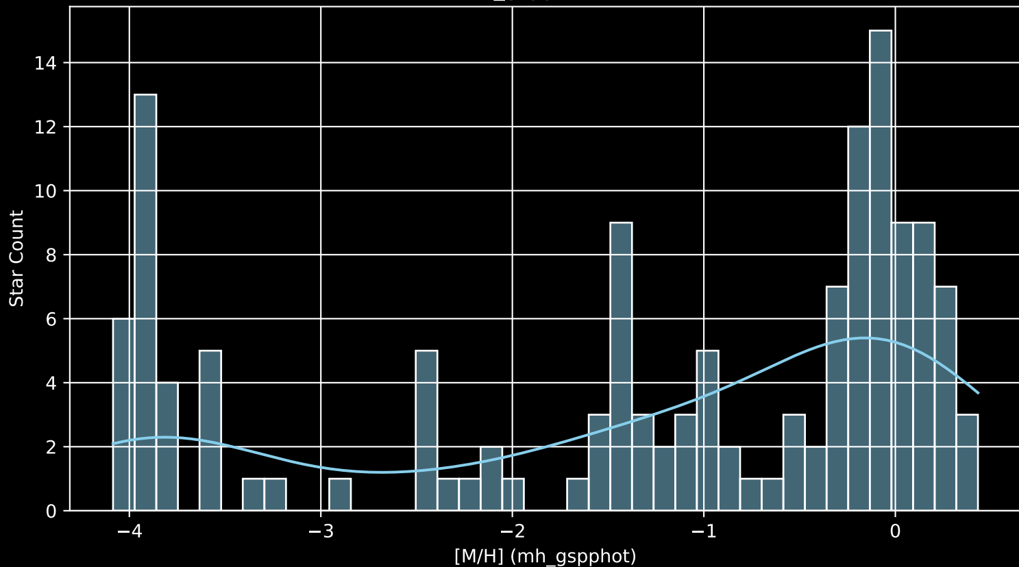
APOGEE DR17 Field: [000+05-O [M/H] (mh_gspphot) (n= 138)
