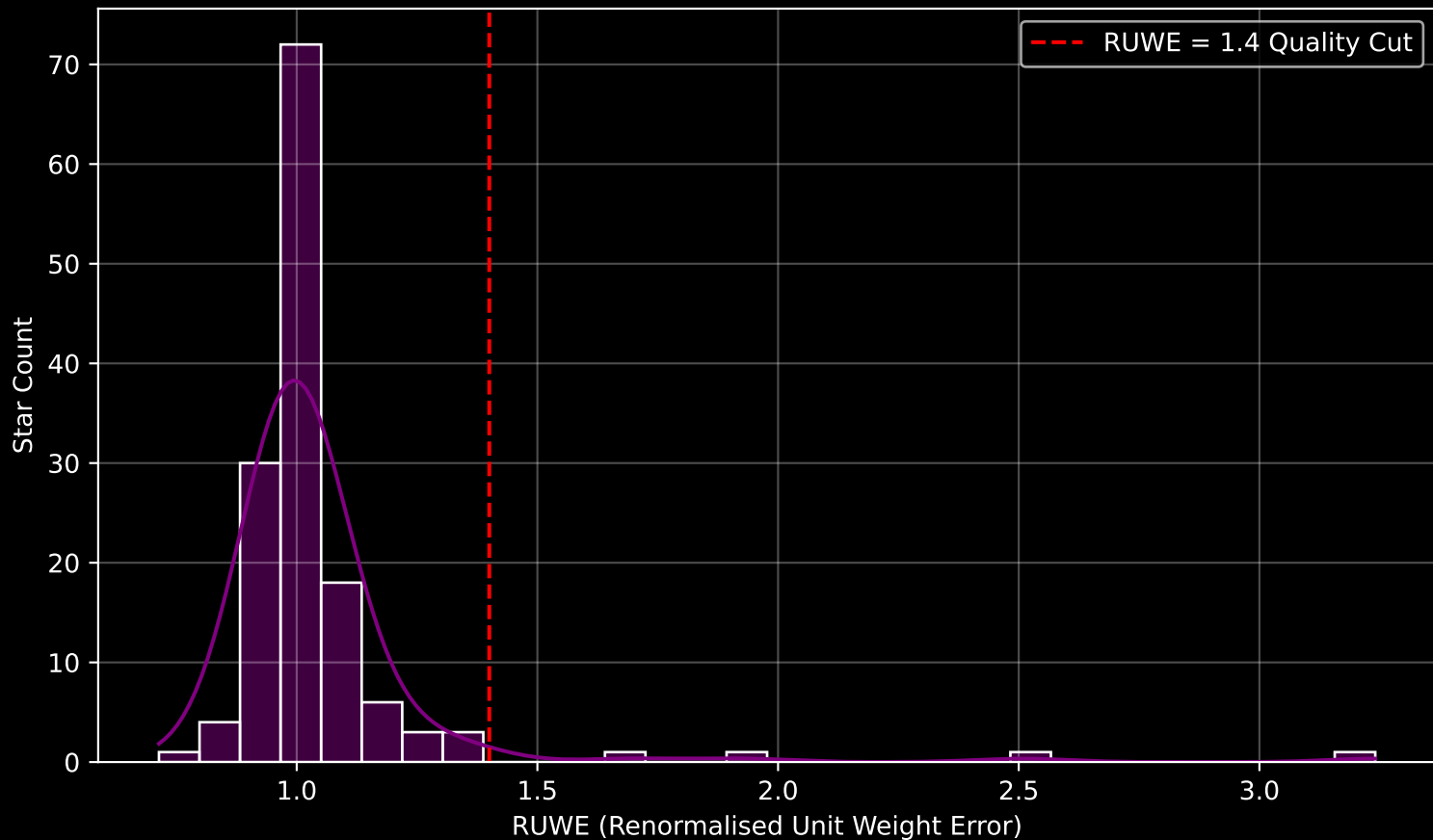
GAPOGEE DR17 Field [000+05-O] RUWE Distribution (n= 141)
