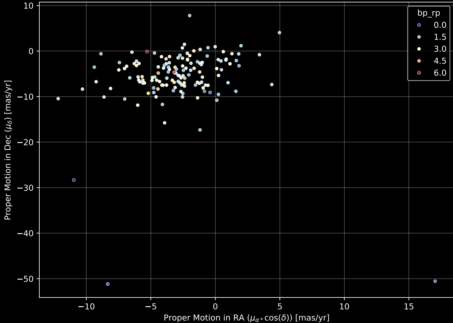
APOGEE DR17 Field: [000+05-O] Proper Motion Diagram (n= 142)
