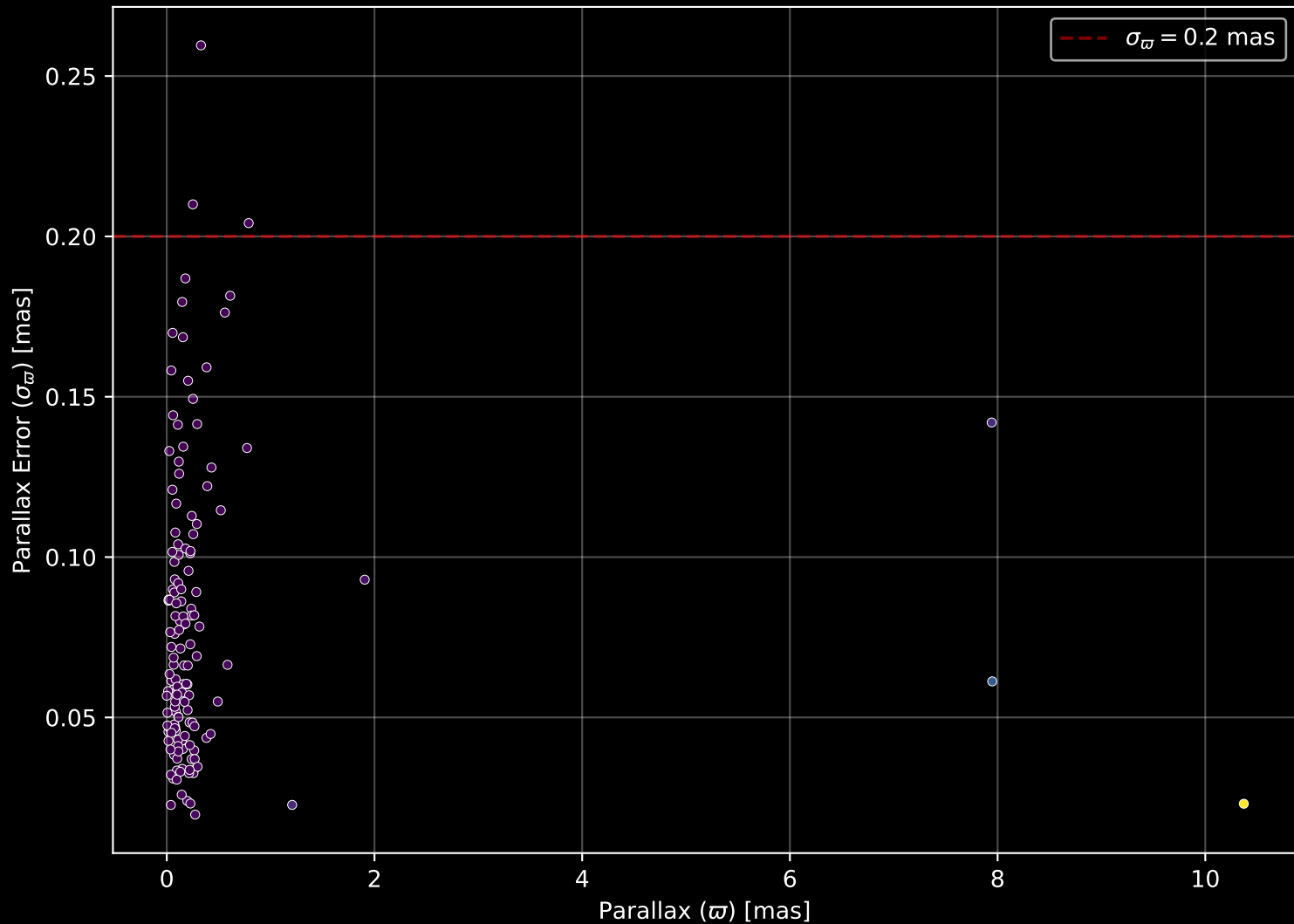
APOGEE DR17 Field: [000+05-O] Parallax Quality (n= 142)
