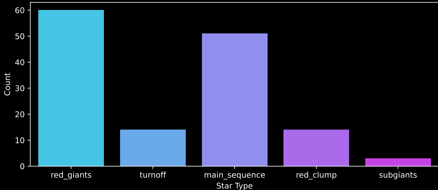
APOGEE DR17 Field: [000+05-O] Count plot of Star Type
