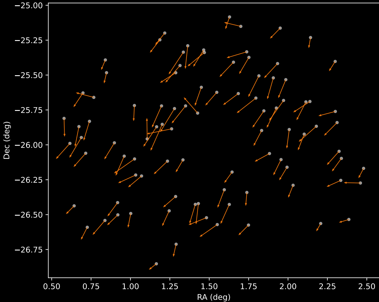
APOGEE DR17 Cluster 2 Proper Motion Vectors (n=91)
